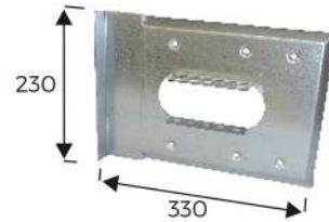
Fixed side plate depth 30mm
