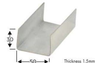
90P06 30x50x30 mm for lower guide
