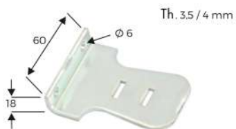
Reinforced iron bumper
