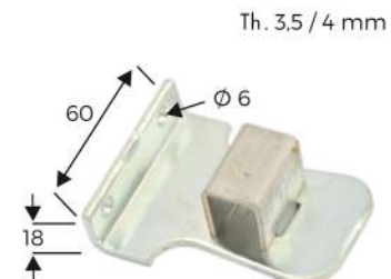
Reinforced iron bumper
