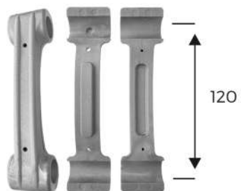
TUB303N InNylon, wheelbase of 120 mm nylon
