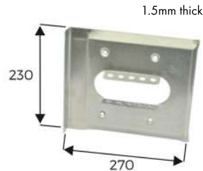
Small fixed side plate depth 30mm
