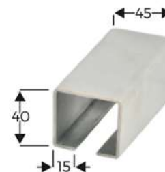
90P04 15x40x45x40x15 mm for upper guide
