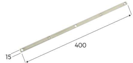
Diagonal with 5 holes
